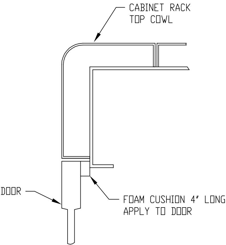
DETAIL "C"
