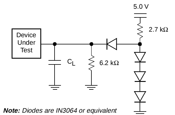
Figure 6. Test Setup
