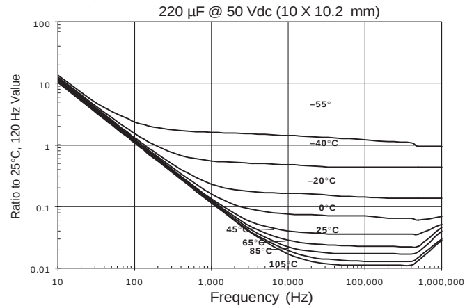
Impedance vs. Temperature and Frequency
