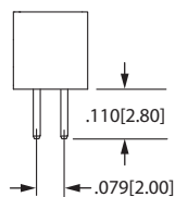
STRAIGHT (ST) Example P/N: SBH21-NBPN-D20-ST-BK
