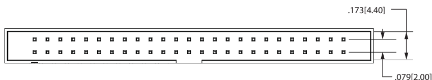
STRAIGHT (ST) Example P/N: SBH21-NBPN-D20-ST-BK
