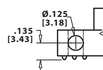
SIDE MOUNTING (S)
