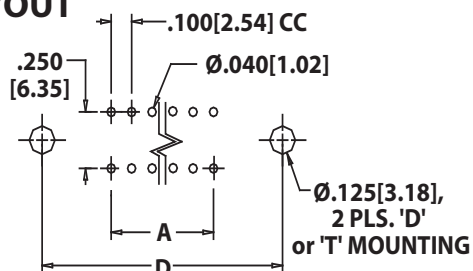
STRAIGHT PIN (RS, RM) TERMINATIONS
