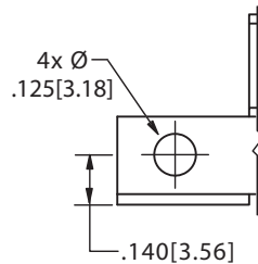
FLUSH, SIDE MOUNTING with CLEARANCE HOLES (Z)
