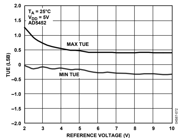
Figure 19. TUE vs. Reference Voltage
