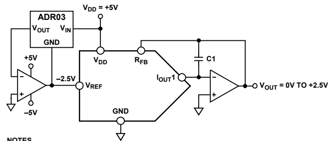
Figure 46. Positive Output Voltage with Minimum Components
