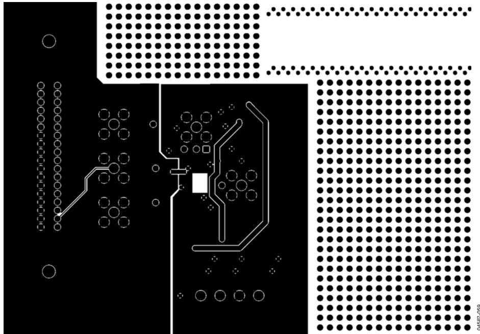
Figure 64. Solder-Side Artwork
