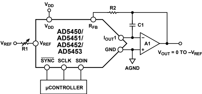
Figure 43. Unipolar Mode Operation
