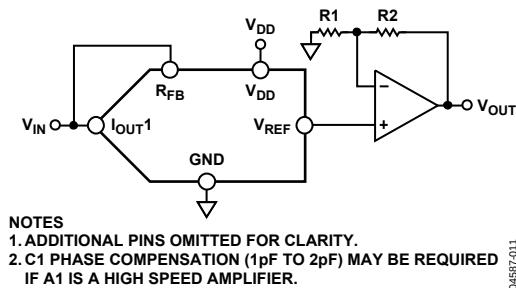
Figure 45. Single-Supply Voltage-Switching Mode
