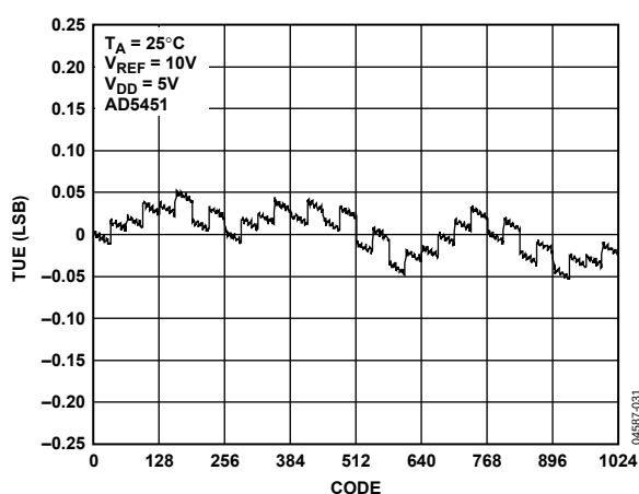
Figure 16. TUE vs. Code (10-Bit DAC)
