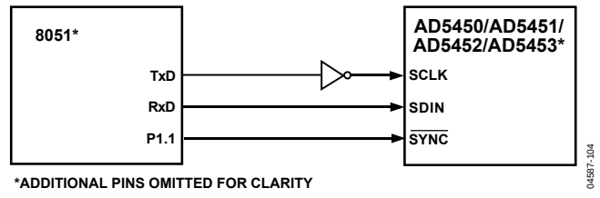
Figure 57. 80C51/80L51-to-AD5450/AD5451/AD5452/AD5453 Interface
