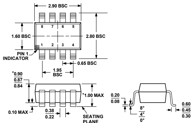
Figure 65. 8-Lead Thin Small Outline Transistor Package [TSOT]
