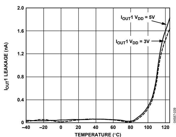
Figure 22. I_{OUT1} Leakage Current vs. Temperature
