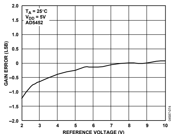
Figure 21. Gain Error (LSB) vs. Reference Voltage
