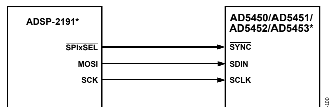
Figure 53. ADSP-2191 SPI-to-AD5450/AD5451/AD5452/AD5453 Interface
