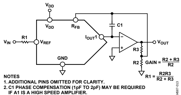
Figure 47. Increasing Gain of Current-Output DAC
