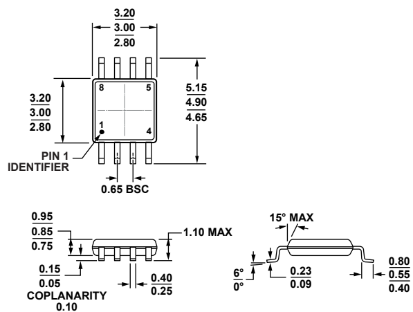
Figure 66. 8-Lead Mini Small Outline Package [MSOP]
