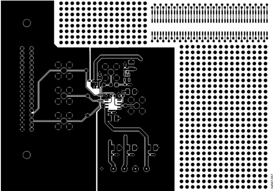
Figure 62. Component-Side Artwork
