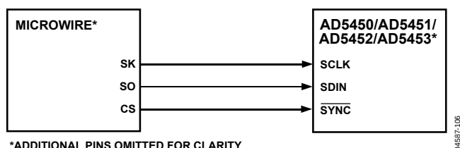
Figure 59. MICROWIRE-to-AD5450/AD5451/AD5452/AD5453 Interface
