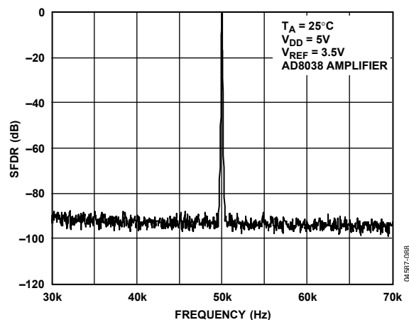
Figure 38. Narrow-Band SFDR, f_{OUT} = 50\text{ kHz} , Clock = 1 MHz
