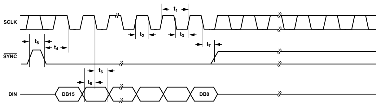
Figure 2. Timing Diagram
