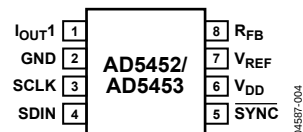
Figure 4. MSOP Pin Configuration
