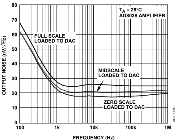
Figure 41. Output Noise Spectral Density
