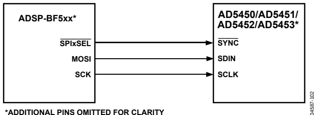
Figure 55. ADSP-BF5xx-to-AD5450/AD5451/AD5452/AD5453 Interface
