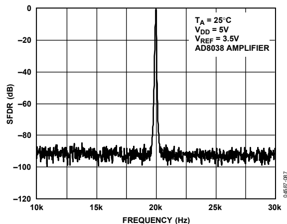
Figure 37. Narrow-Band SFDR, f_{OUT} = 20\text{ kHz} , Clock = 1 MHz
