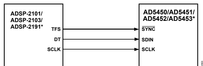
Figure 54. ADSP-2101/ADSP-2103/ADSP-2191* SPORT-to-AD5450/AD5451/AD5452/AD5453 Interface
