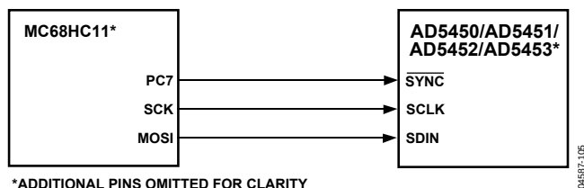
Figure 58. MC68HC11-to-AD5450/AD5451/AD5452/AD5453 Interface
