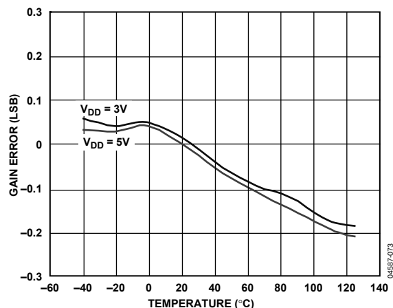
Figure 20. Gain Error (LSB) vs. Temperature
