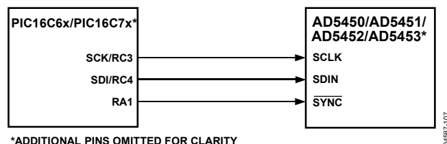
Figure 60. PIC16C6x/7x-to-AD5450/AD5451/AD5452/AD5453 Interface
