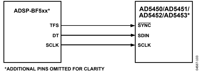
Figure 56. ADSP-BF5xx SPORT-to-AD5450/AD5451/AD5452/AD5453 Interface
