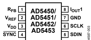
Figure 3. TSOT Pin Configuration
