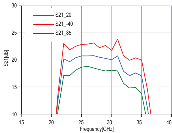
Figure 11. Typical Gain over temperature
