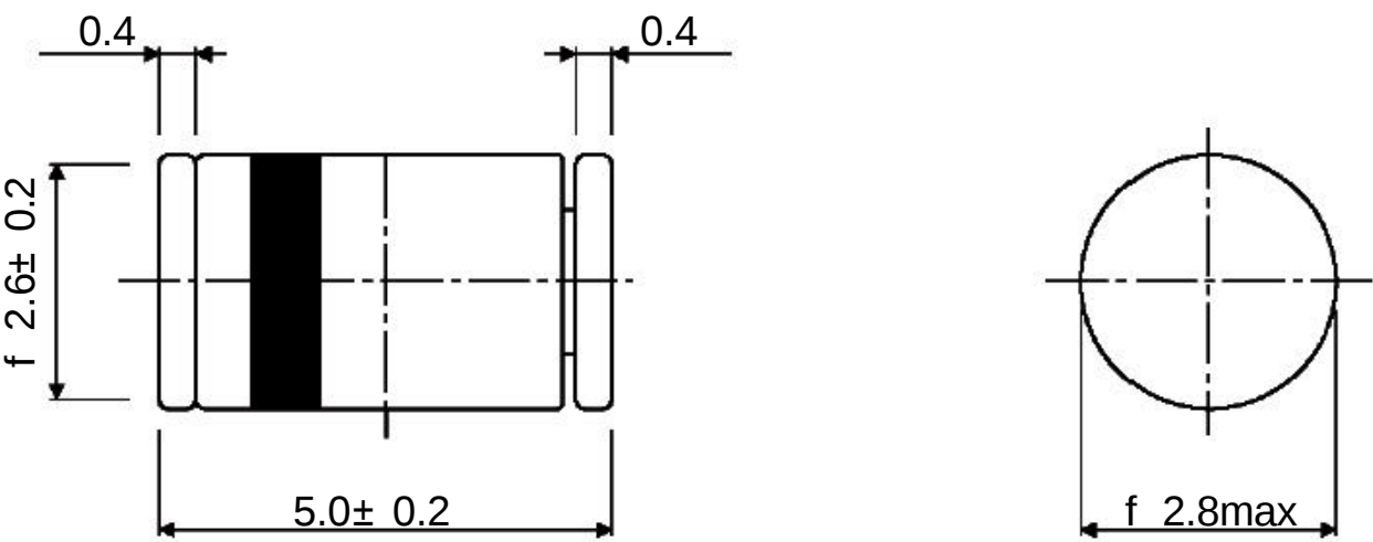
Standard Glass Case JEDEC LL 41
