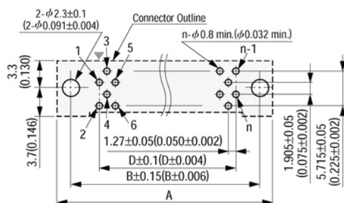
For 20,32,40,52,60,68,80,100 contacts
