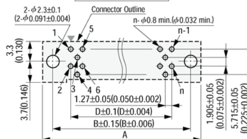
For 26,30,34,50 contacts
