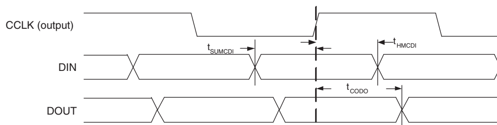
Figure 3-14. sysCONFIG Master Serial Port Timing
