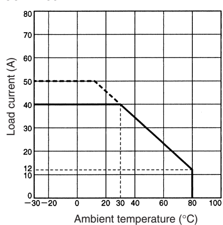
G3PA-450B-VD-2
