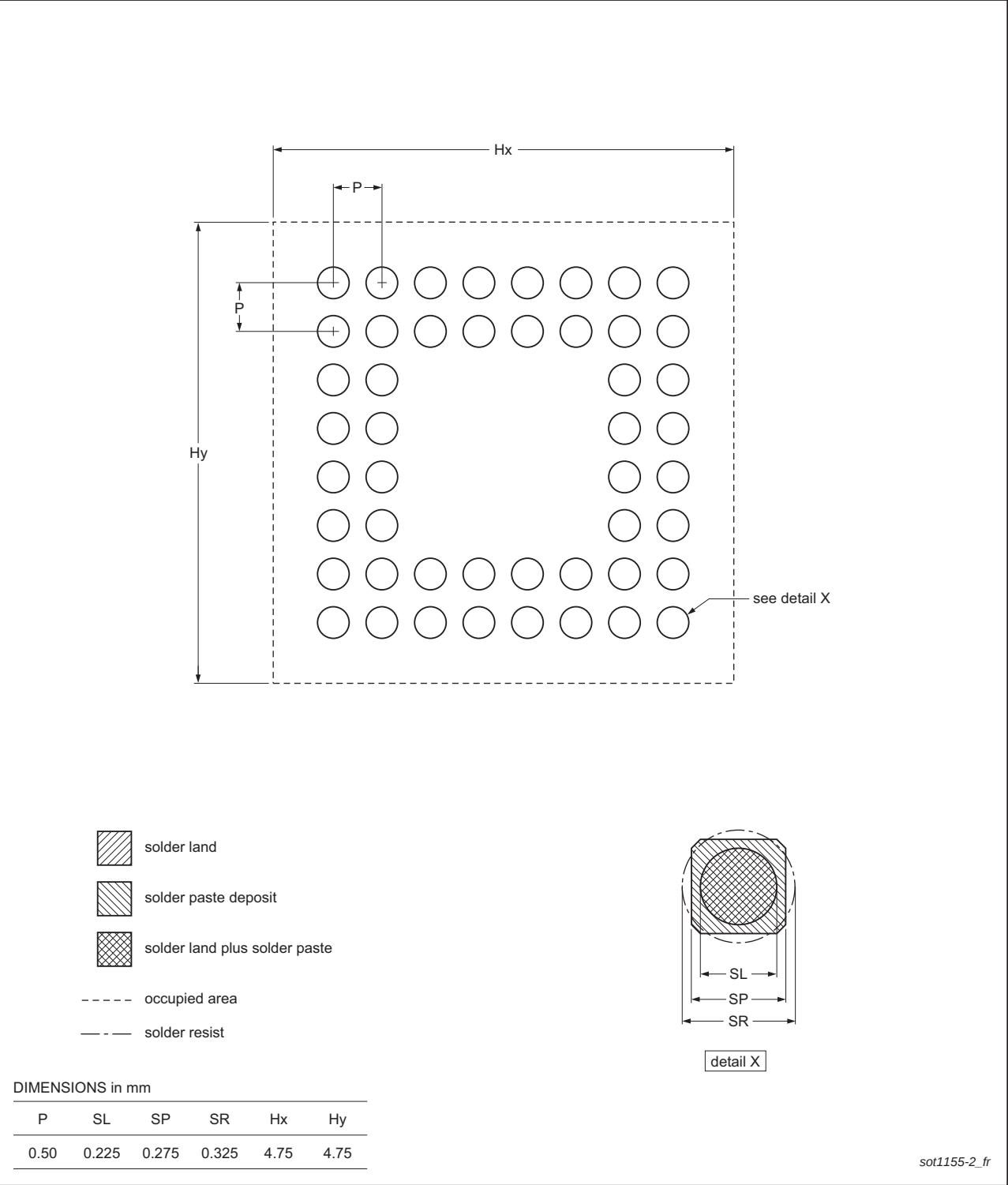
Fig 42. Reflow soldering for the TFBGA48 package
