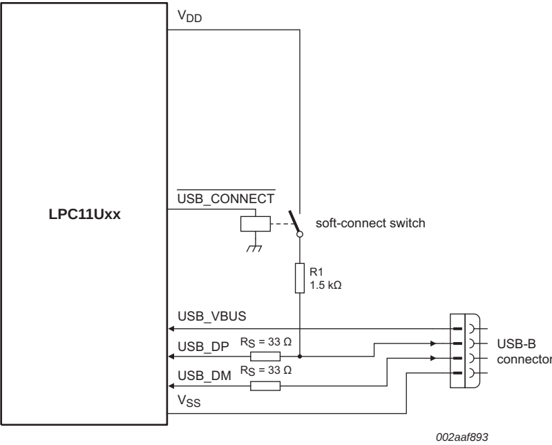
Fig 29. USB interface with soft-connect
