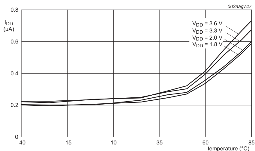
Fig 14. Typical supply current versus temperature in Deep power-down mode
