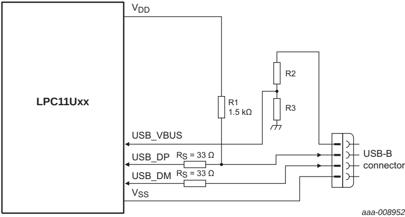
Fig 28. USB interface on a bus-powered device where USB_VBUS = 5 V, VDD not present
