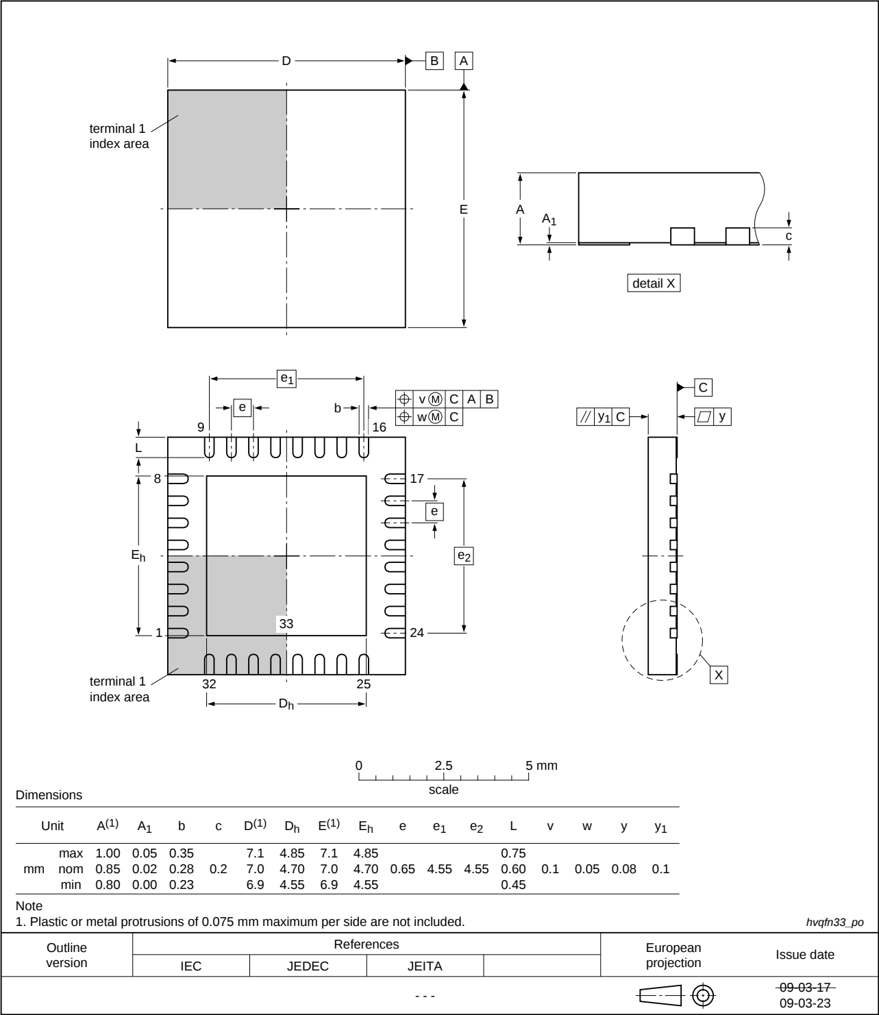
Fig 36. Package outline HVQFN33 (7 x 7 x 0.85 mm)
