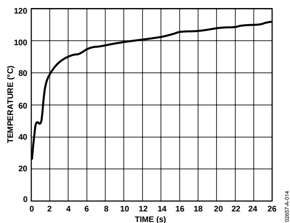
Figure 14. Response to Thermal Shock
