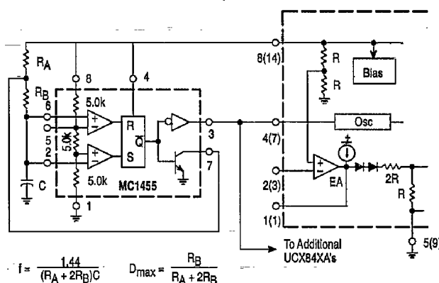
Figure 18. External Duty Cycle Clamp and Multi-Unit Synchronization
