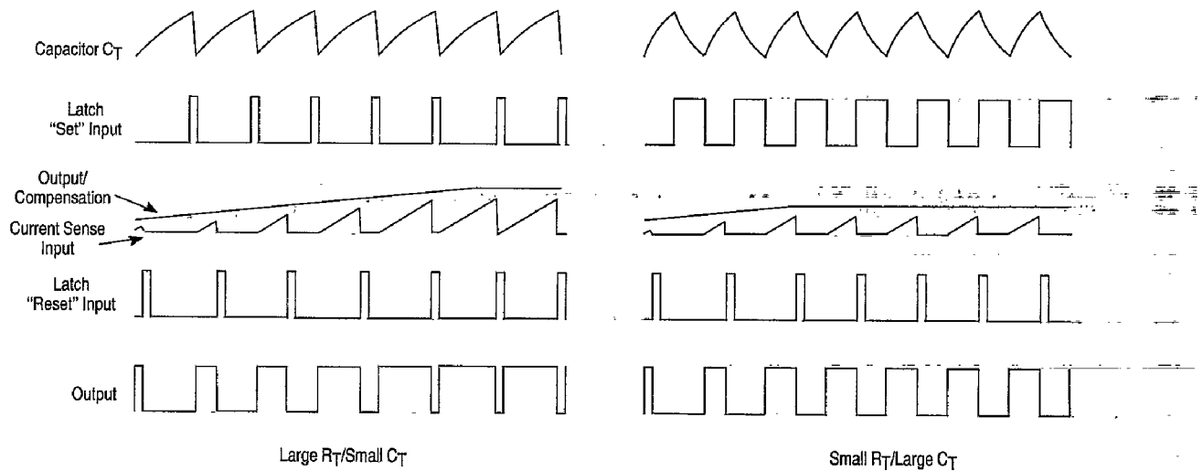
Figure 16. Timing Diagram
