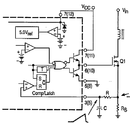
Figure 23. Current Waveform Spike Suppression
