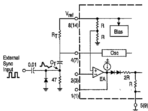
Figure 17. External Clock Synchronization
