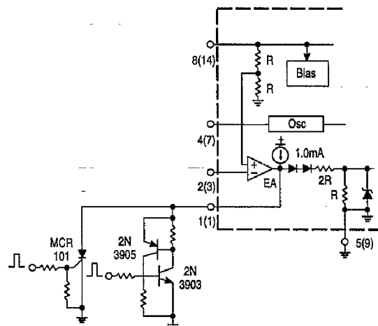
Figure 27. Latched Shutdown
