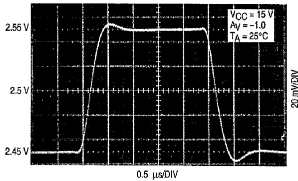
Figure 3. Error Amp Small Signal Transient Response
