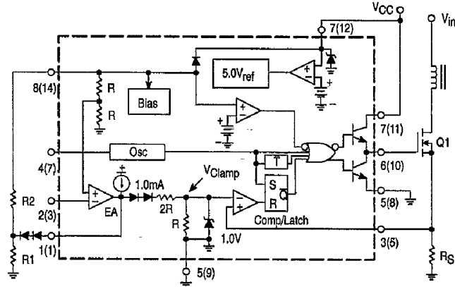
Figure 19. Adjustable Reduction of Clamp Level
