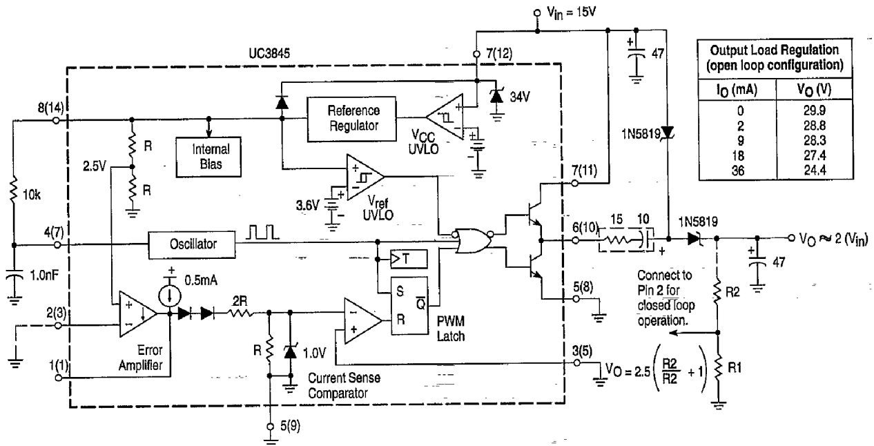
Figure 30. Step-Up Charge Pump Converter
