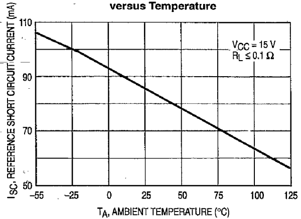
Figure 8. Reference Short Circuit Current versus Temperature
