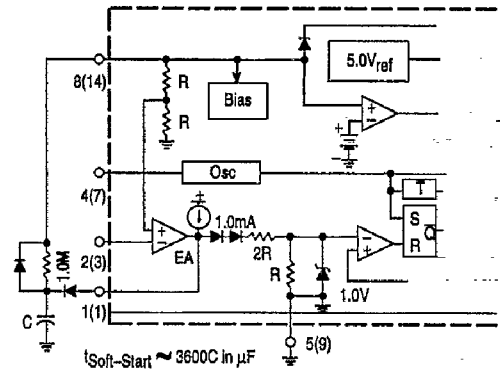
Figure 20. Soft-Start Circuit
