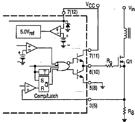
Figure 24. MOSFET Parasitic Oscillations
