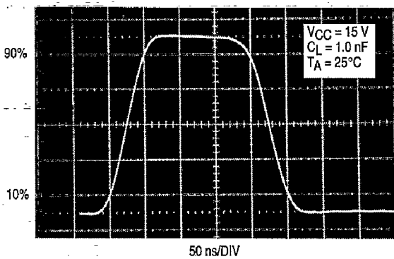
Figure 12. Output Waveform
