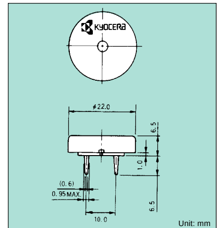
KBS-20DB-3P-0 / KBS-20DB-4P-0 / KBS-20DB-6P-0
