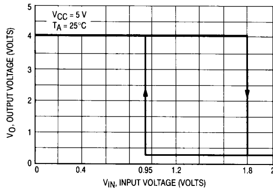
Figure 2. V_{IN} versus V_{OUT} Transfer Function
