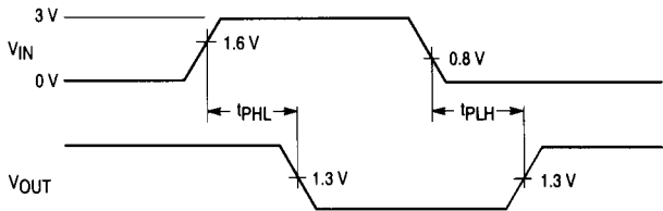
Figure 1. AC Waveforms
