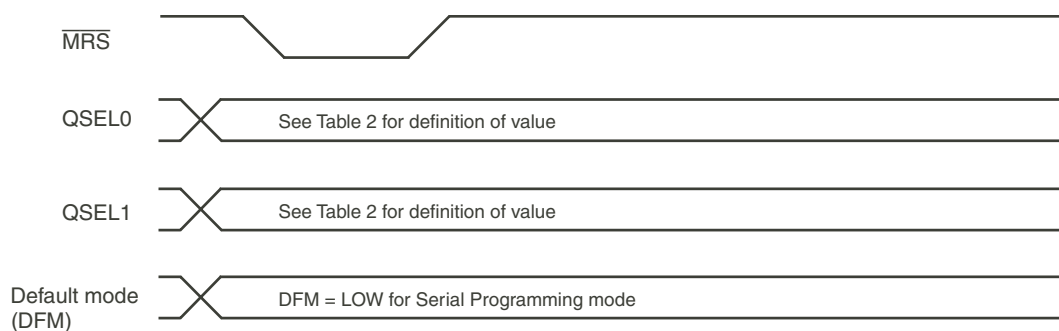
Figure 3. Reference Signals
