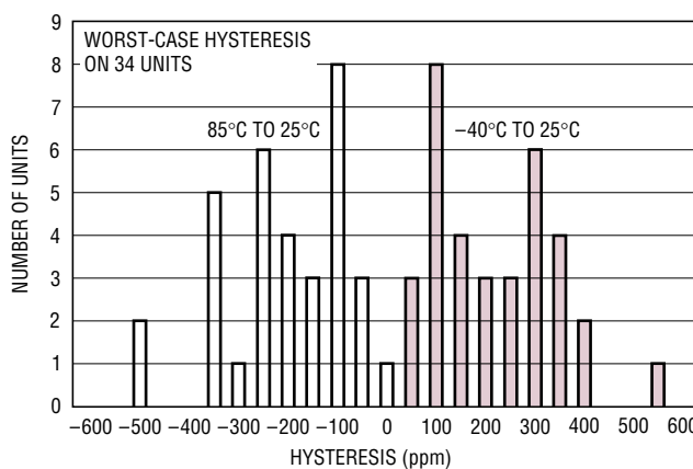
Figure 7. –40°C to 85°C Hysteresis
