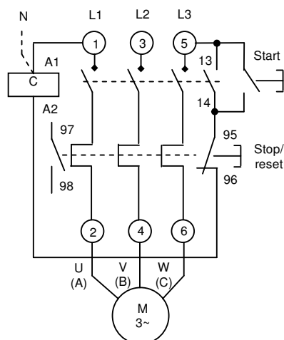
Standard circuit
