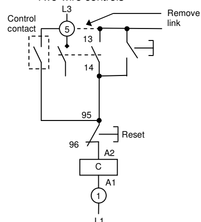
Two-wire controls
