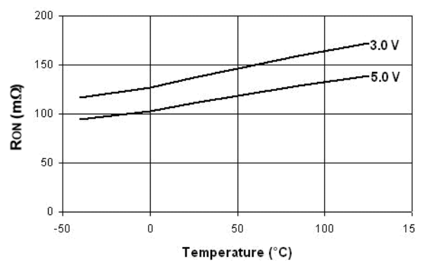
Figure 47. R_{ON} vs. temperature (STMPS2161/2171)
