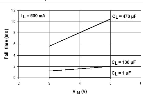
Figure 51. Output fall time vs. V_{IN} (STMPS2161/2171)
