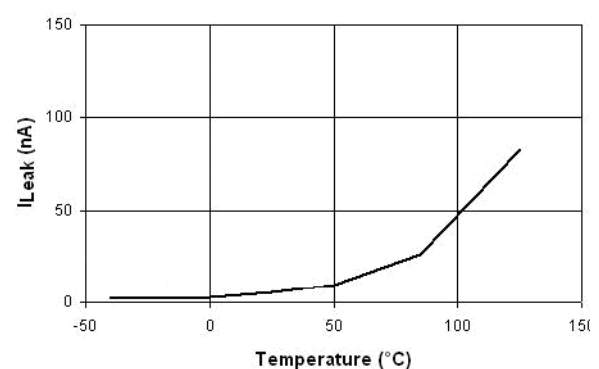
Figure 49. Switch leakage vs. temperature (STMPS2161/2171)
