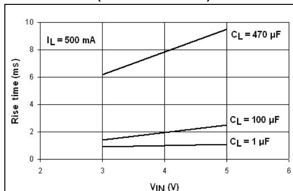
Figure 50. Output rise time vs. V_{IN} (STMPS2161/2171)
