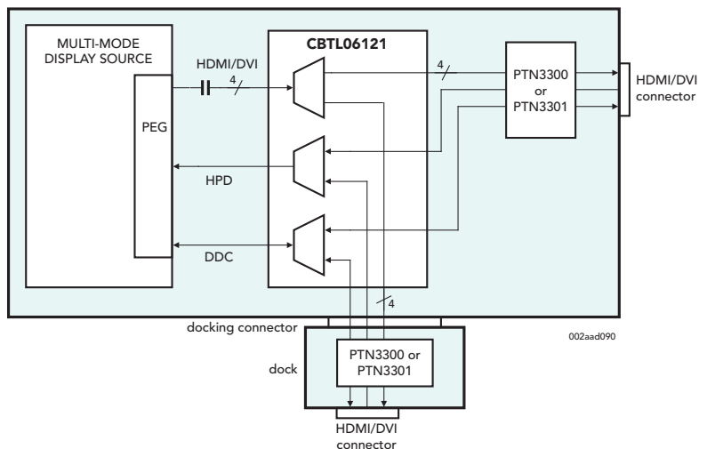
HDMI/DVI docking solution for mobile platform
