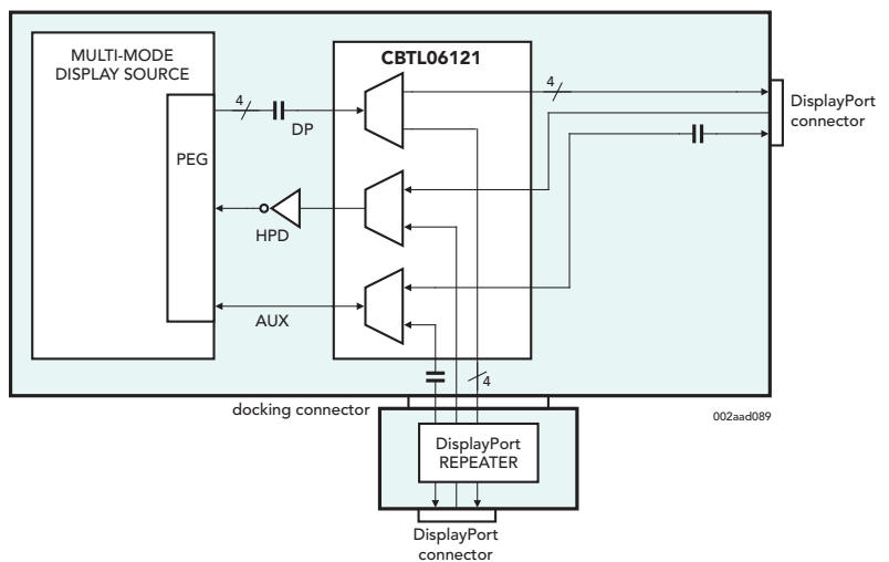
DisplayPort docking solution for mobile platform
