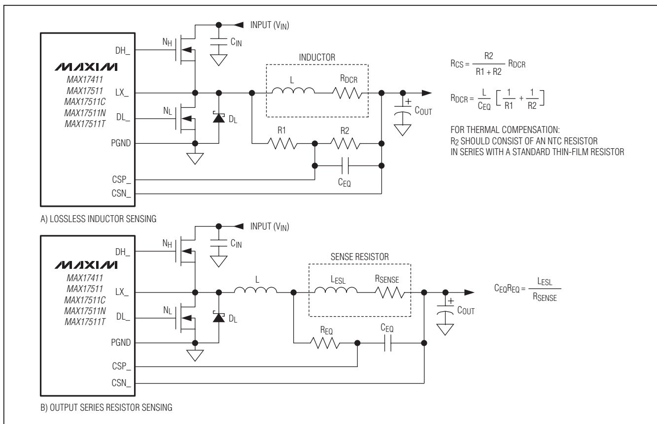
Figure 6. Current-Sense Methods
