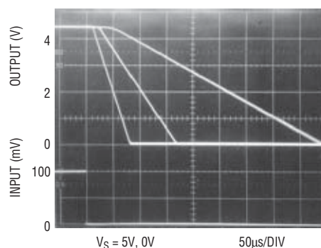
V_S = 5V, 0V
