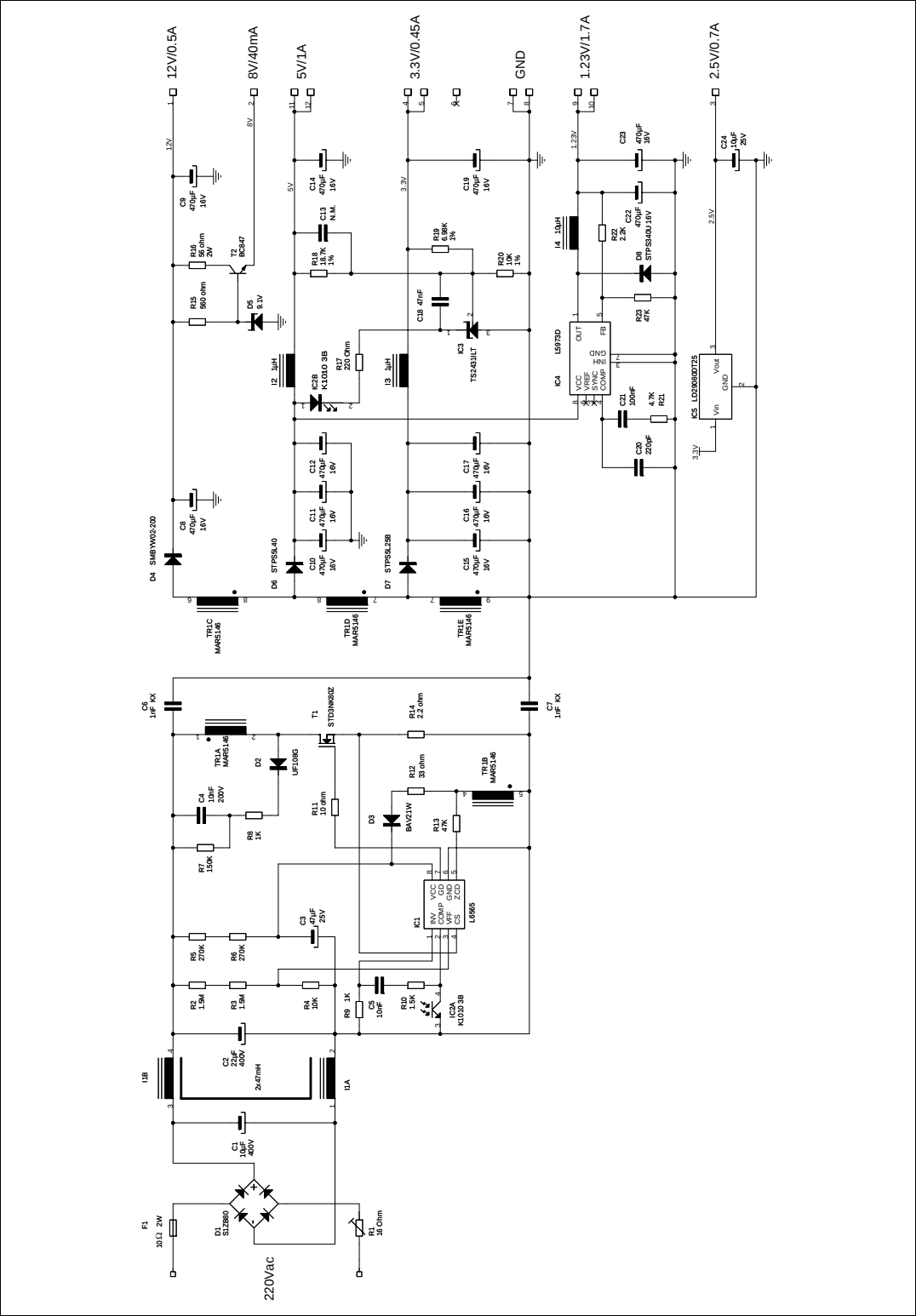
Figure 1. Board schematic
