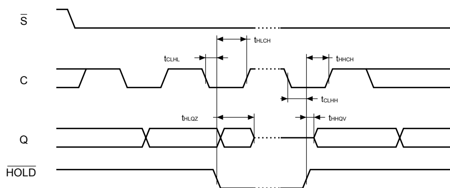
Figure 20. Hold timing
