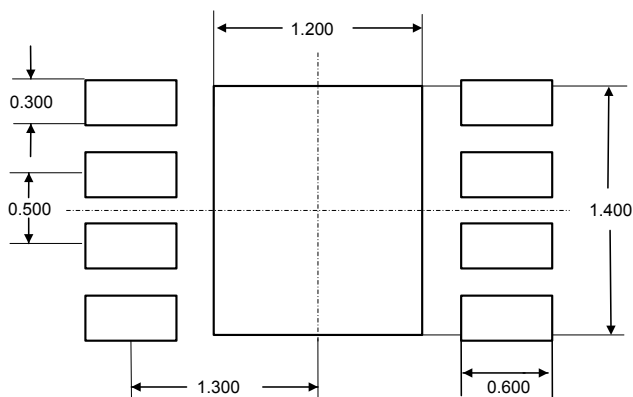
Figure 27. WFDFPN8 (DFN8) – Footprint example
