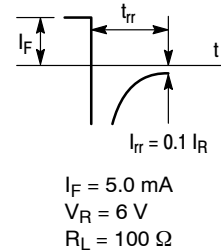
OUTPUT PULSE
