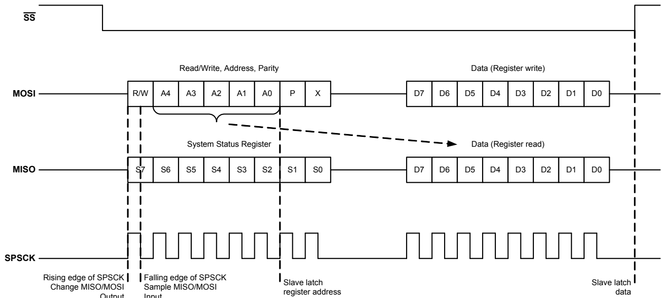
Figure 9. SPI Protocol
