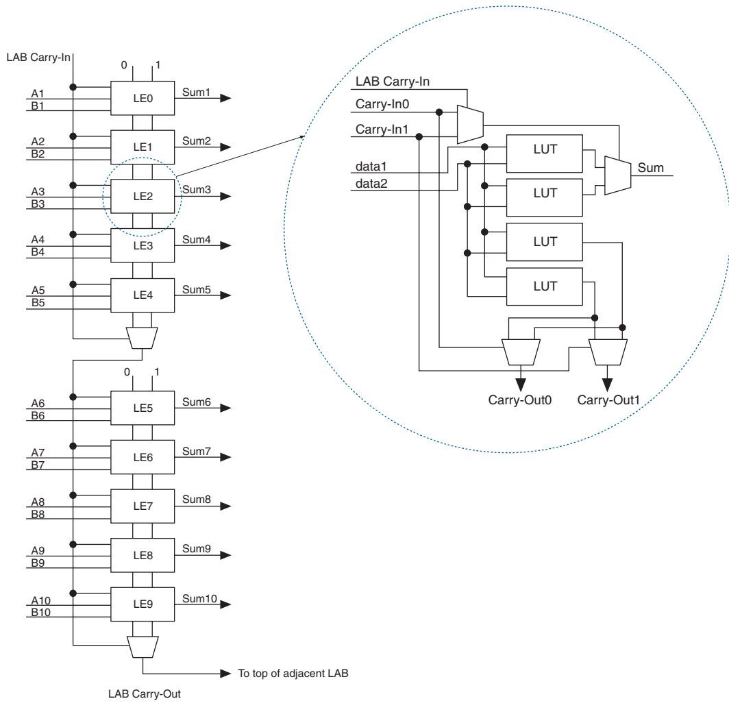
Figure 2–9. Carry-Select Chain
