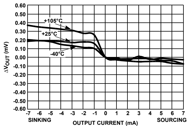
FIGURE 106. LOAD REGULATION
