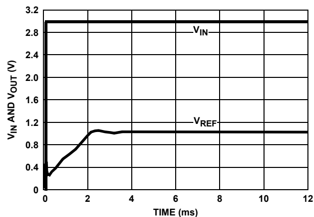
FIGURE 12. TURN-ON TIME ( +25^\circ C )
