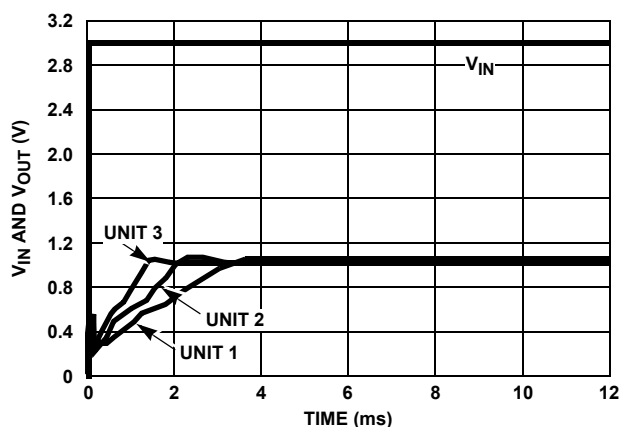
FIGURE 11. TURN-ON TIME ( +25^\circ C )
