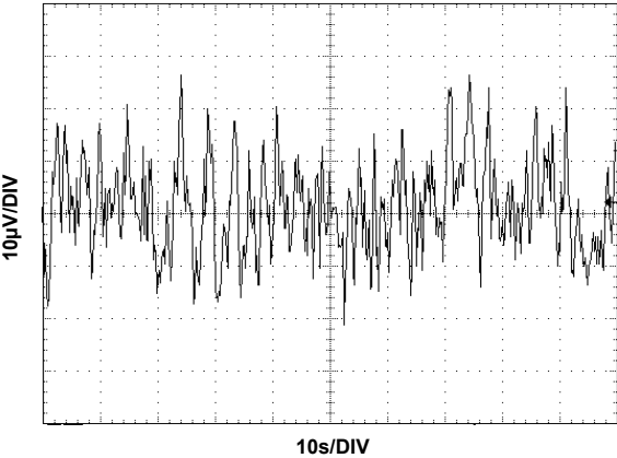
FIGURE 27. V_{OUT} NOISE
