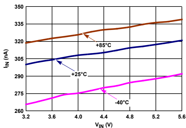
FIGURE 84. I_{IN} vs V_{IN} OVER-TEMPERATURE
