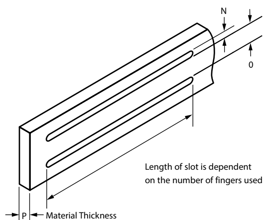
RH Mounting Hole Pattern
