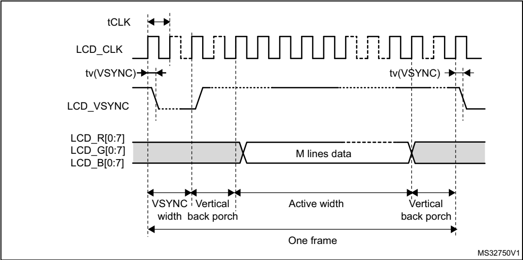
Figure 52. LCD-TFT vertical timing diagram
