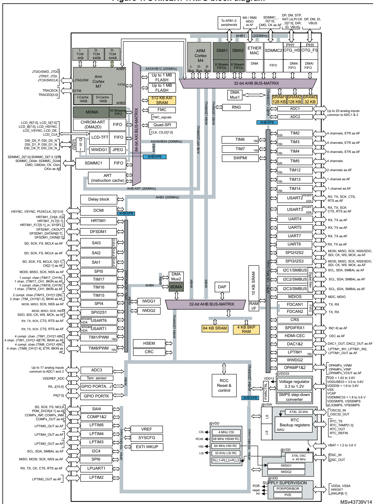
Figure 1. STM32H747xl/G block diagram
