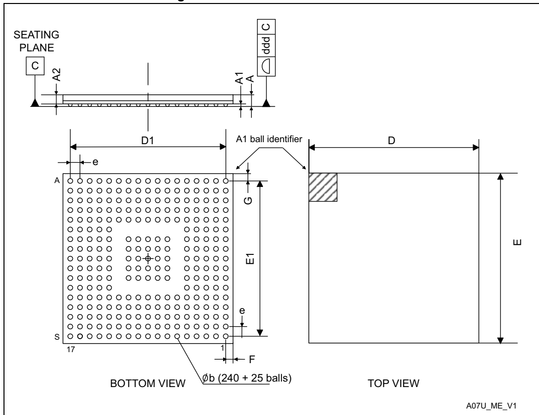
Figure 81. TFBGA240+25 - Outline
