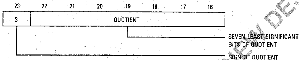
Figure 5. Quotient Byte
