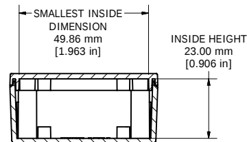
SECTION W-W
