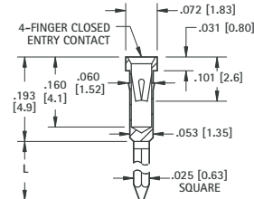
IC SOCKET CONTACTS FOR .015 (.38) - .025 (.64) LEADS - PRESS-FIT
