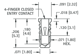
.032 (.81) - .046 (1.17) PIN - PRESS-FIT
