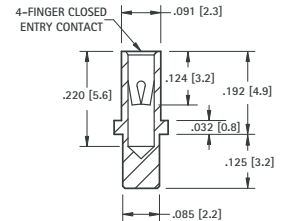
.032 (.81) - .046 (1.17) PIN - SOLDER MOUNT
