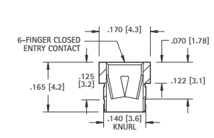
.084 (2.13) - .102 (2.6) PIN - PRESS-FIT
