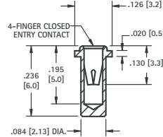
.032 (.81) - .046 (1.17) PIN - SOLDER MOUNT
