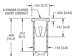
.065 (1.65) - .082 (2.08) PIN - SOLDER MOUNT
