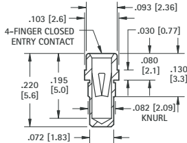
.032 (.81) - .046 (1.17) PIN - PRESS-FIT
