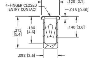
.048 (1.22) - .064 (1.63) PIN - SOLDER MOUNT
