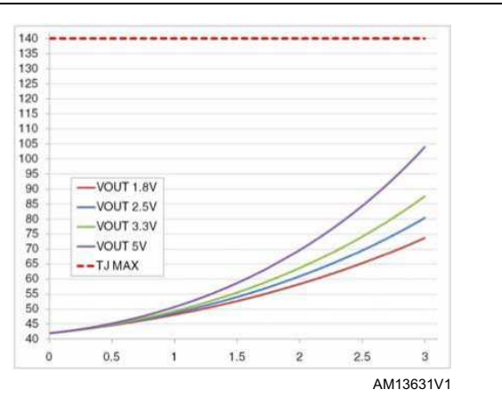
Figure 37. T_J vs. I_{\text{OUT}} ( V_{\text{IN}} 12\text{V} )
