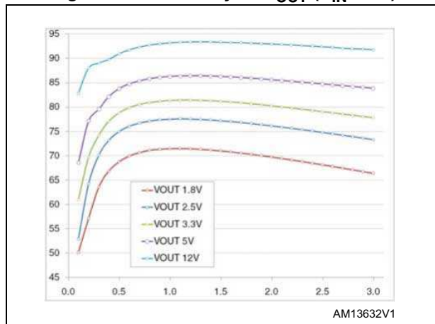
Figure 38. Efficiency vs. I_{\text{OUT}} ( V_{\text{IN}} 24\text{V} )
