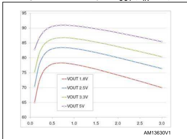
Figure 36. Efficiency vs. I_{\text{OUT}} ( V_{\text{IN}} 12\text{V} )
