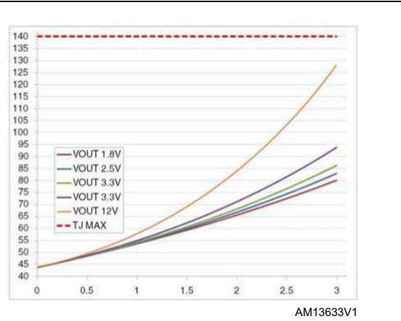
Figure 39. T_J vs. I_{\text{OUT}} ( V_{\text{IN}} 24\text{V} )
