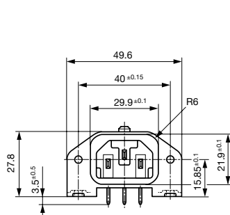
without insulation cover
