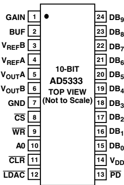
AD5333 PIN CONFIGURATION
