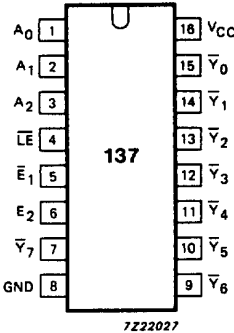
Fig.1 Pin configuration.
