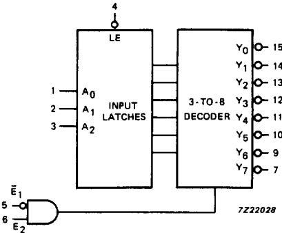
Fig.2 Logic symbol.
