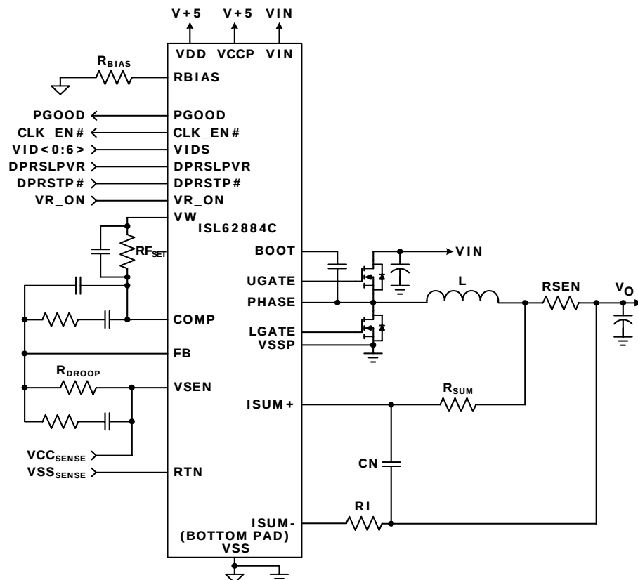
FIGURE 2. ISL62884C TYPICAL APPLICATION CIRCUIT USING RESISTOR SENSING
