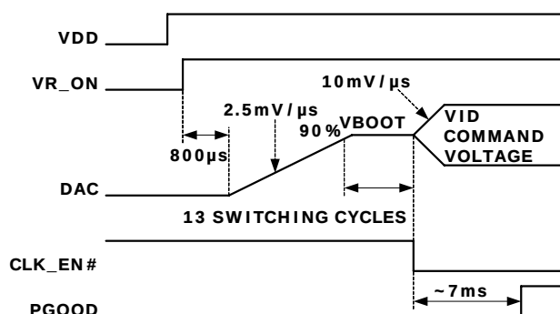
FIGURE 8. SOFT-START WAVEFORMS FOR CPU VR APPLICATION
