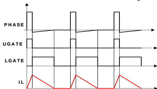
FIGURE 6. DIODE EMULATION
