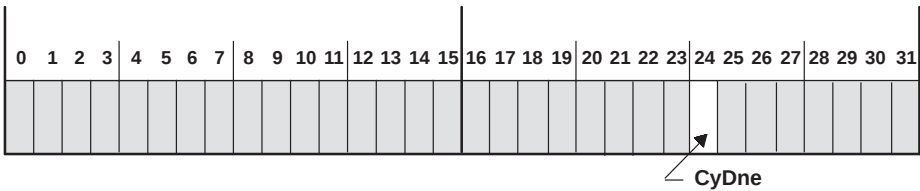
Figure 4–8. CycleMark Format
