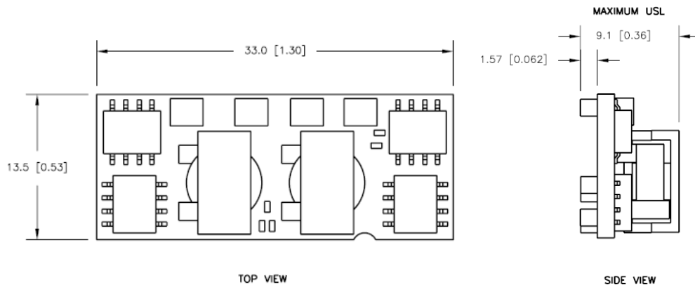
SIDE VIEW
