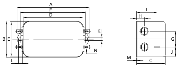
Connection style -06, 20A types
