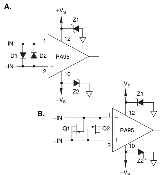
FIGURE 1. OVERVOLTAGE PROTECTION
