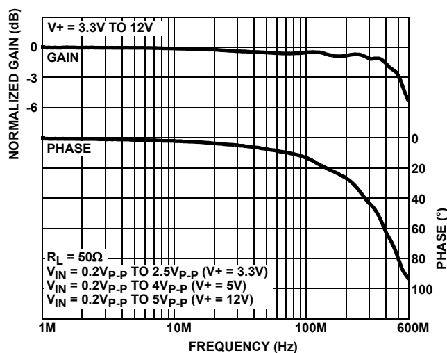
FIGURE 16. FREQUENCY RESPONSE
