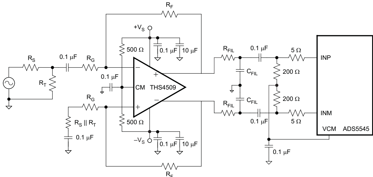
Figure 48. Drive Circuit Using the THS4509
