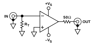
Inverting Configuration
