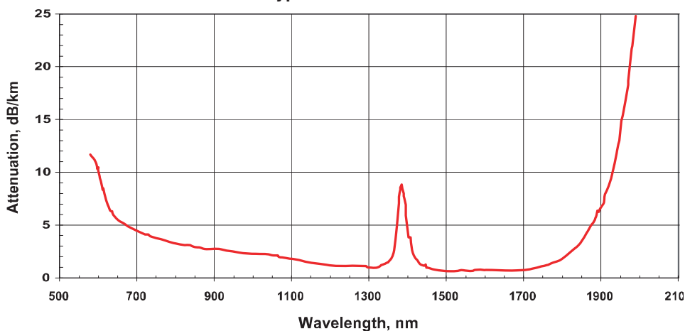
Typical Attenuation
