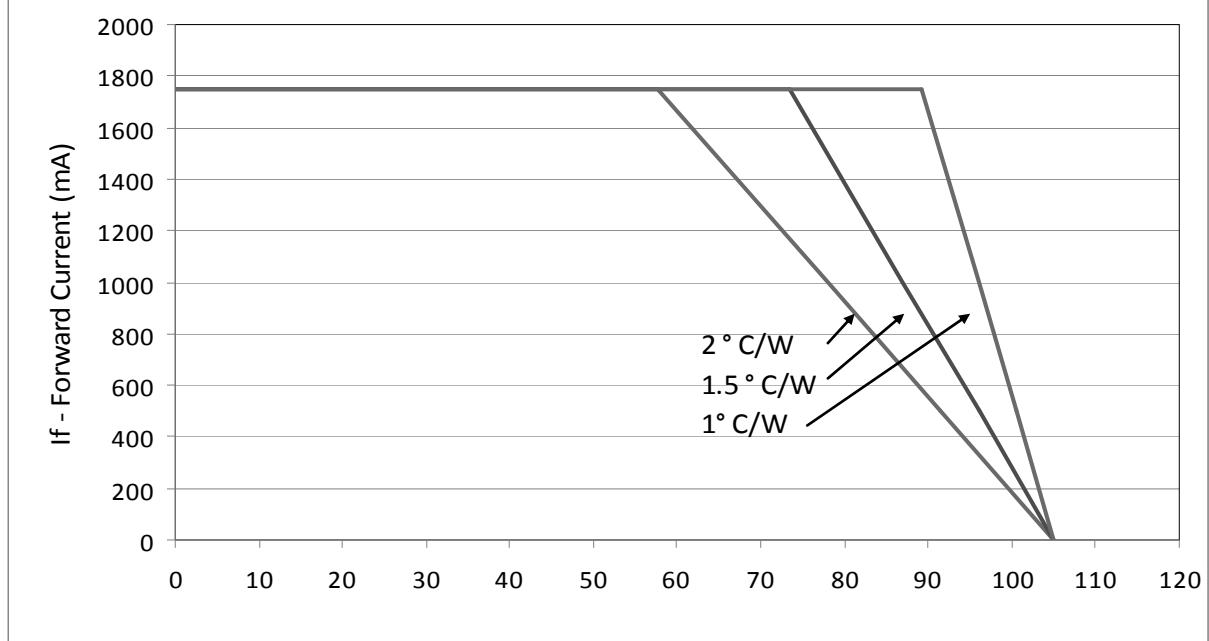
Figure 29: Derating Curve for BXRA-C2000, 1750 mA Drive Current
