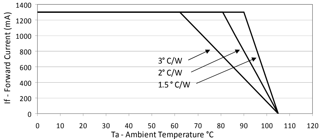
Figure 24: Derating Curve for BXRA-W0800, 1300 mA Drive Current
