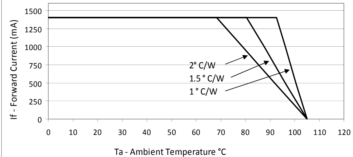
Figure 28: Derating Curve for BXRA-N1200, 1400 mA Drive Current
