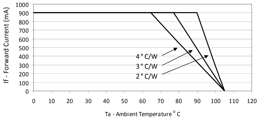
Figure 25: Derating Curve for BXRA-C0800, 900 mA Drive Current
