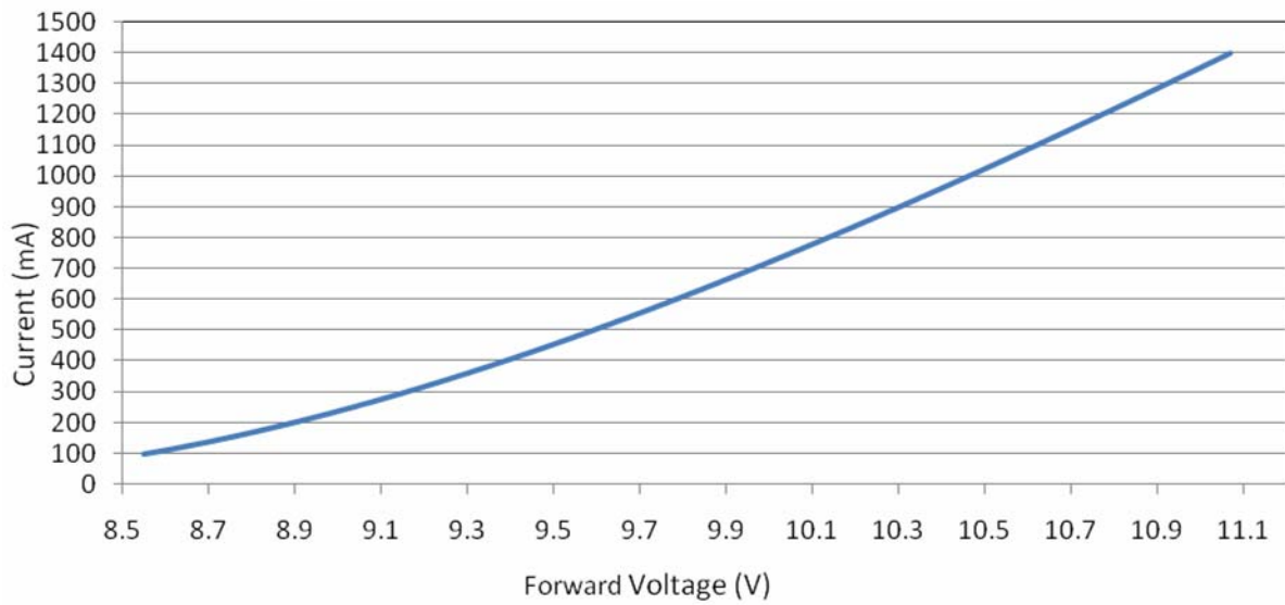
Figure 15: Typical Current vs. Voltage, BXRA-C0400
