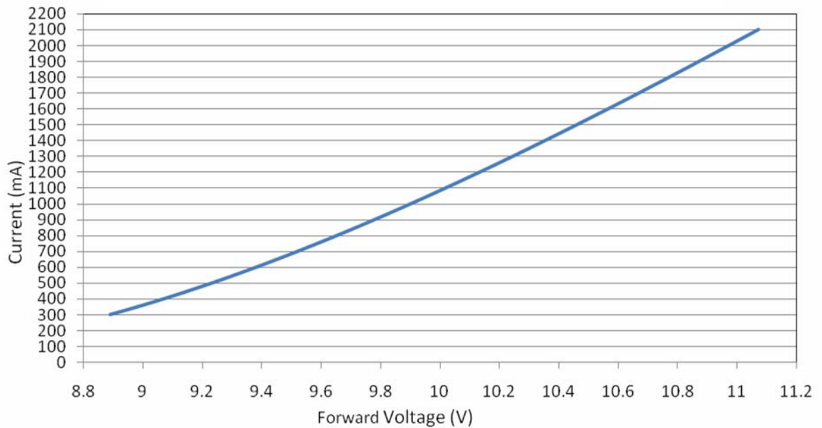
Figure 16: Typical Current vs. Voltage, BXRA-N0400 and BXRA-W0400
