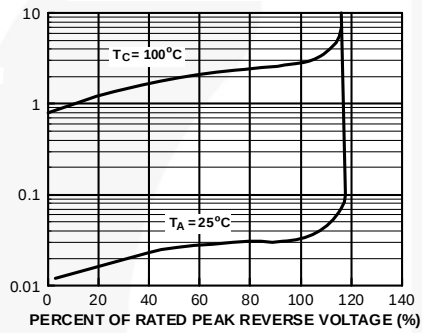
Figure 3. Reverse Characteristics
