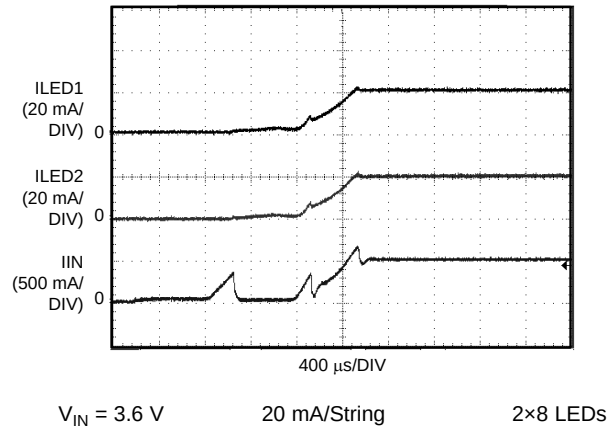
Figure 19. Start-Up Response
