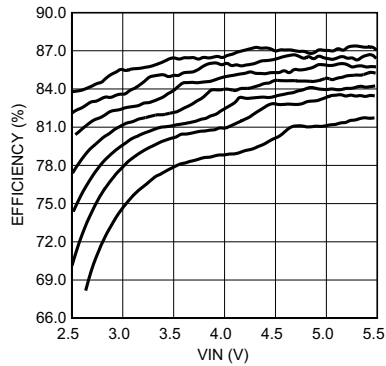
Figure 44. Efficiency vs V_{IN} , Single String
