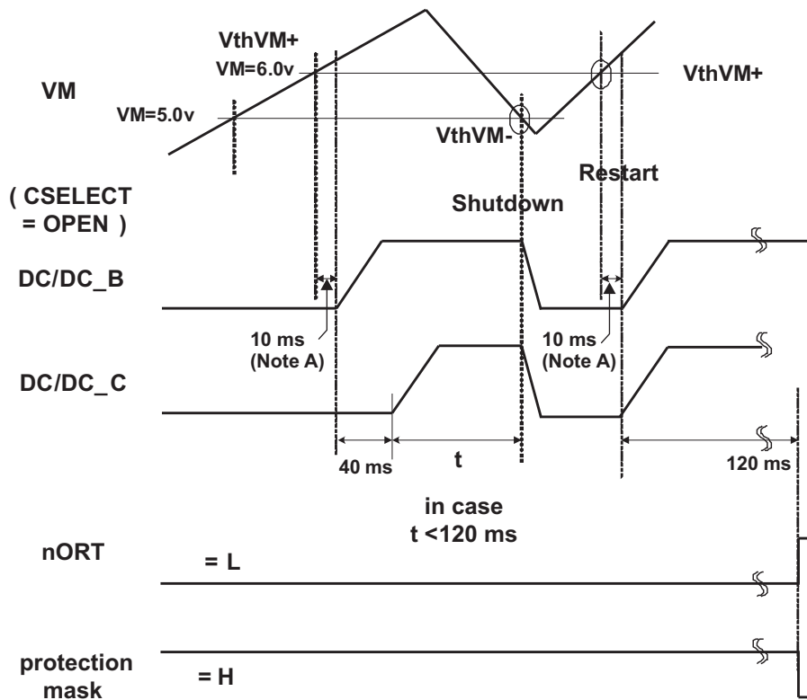
Figure 30. Power Down (Glitch on V_M )
