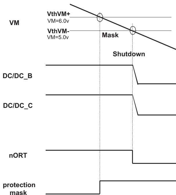
Figure 29. Power Down (Normal)
